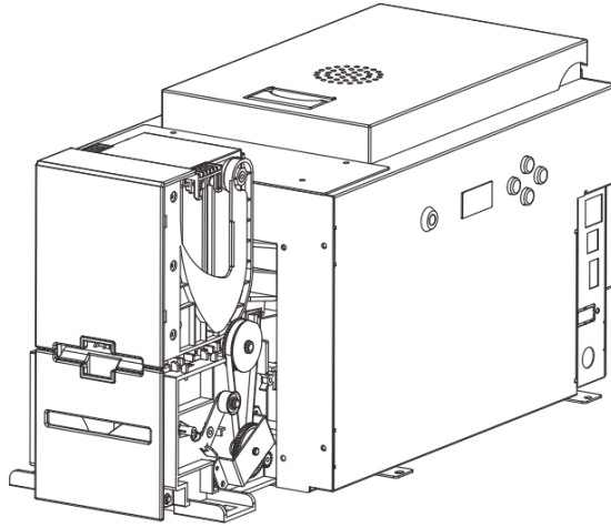
Front view of the printer with a duplex option
